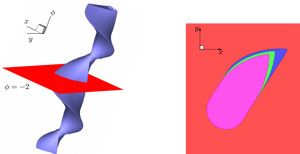
Figure 5: To the left. The solvability set for the case of the absence of the state constraint (blue) and the cutting plane \phi = -2 (red). To the right. The cross sections of three solvability sets computed: a) without the state constraint (the largest one); b) with the state constraint corresponding to s = 1 (the middle one); and c) with the state constraint corresponding to s = 0.8 (the smallest one).
