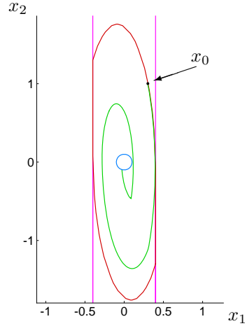
Figure 1: The solvability set (red), the target set (blue), and the optimal trajectory (green).
