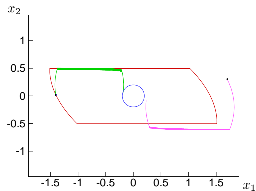
Figure 2: The solvability set (red), the target set (blue), the optimal trajectory for the first player (green), and the win trajectory for the second player (magenta).
