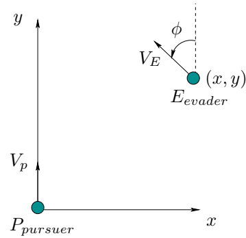
Figure 4: Movable coordinate system. Here, y is the axis collinear to the pursuer's velocity, \phi the angle between the axis y and the evader's velocity, and x is such that \{x, y, \phi\} is the orthogonal right coordinate system.
