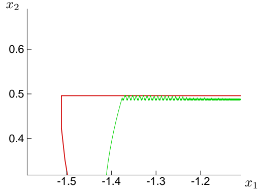
Figure 3: The enlarged fragment of Fig. 2 showing the chattering regime.
